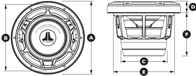
Subwoofer Physical Specifications
